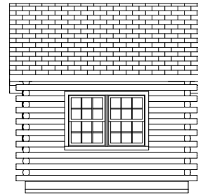
REAR
